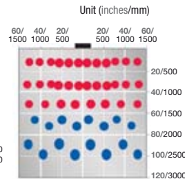
Plan View (Max.)
